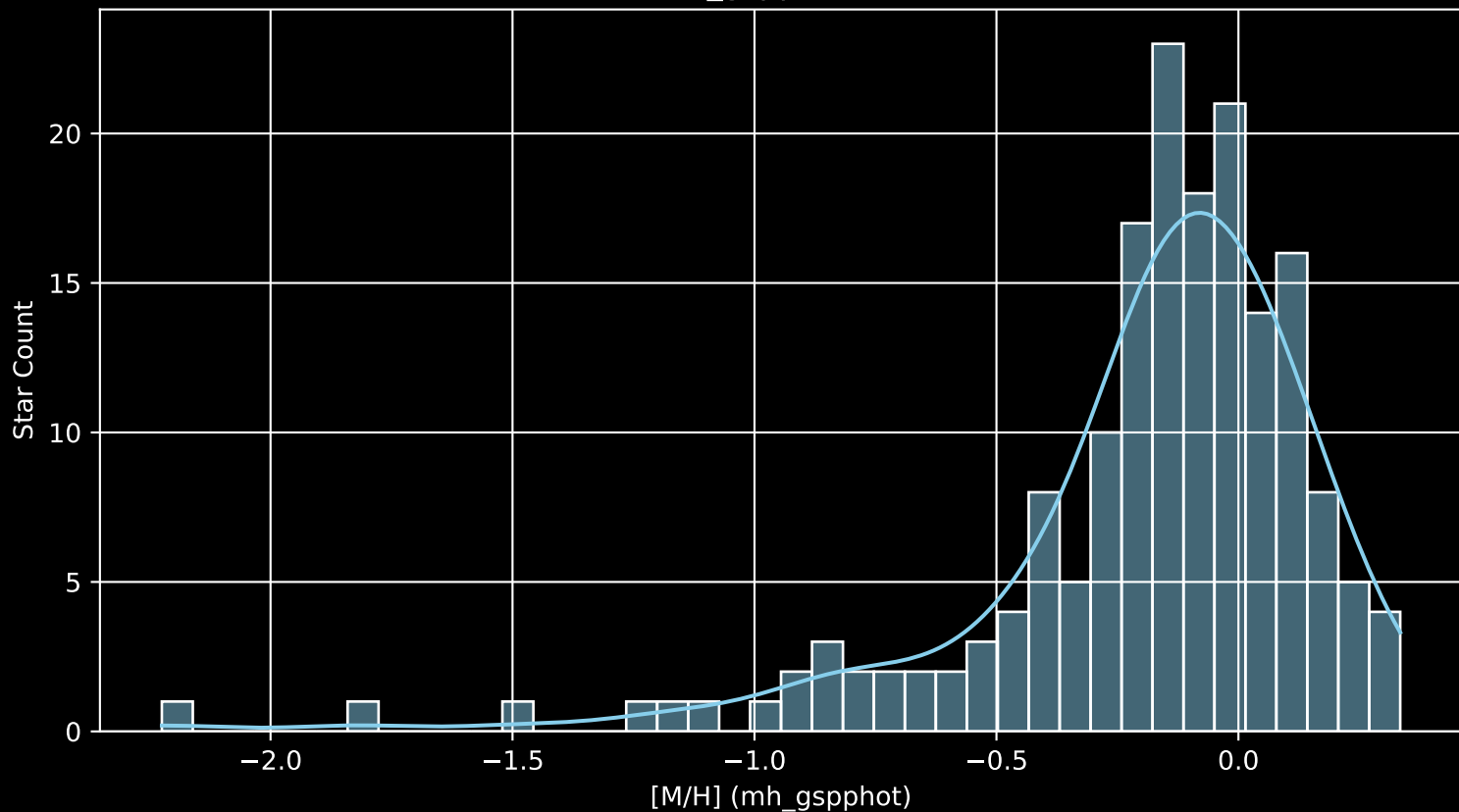
APOGEE DR17 Field: [203-12 [M/H] (mh_gspphot) (n= 176)
