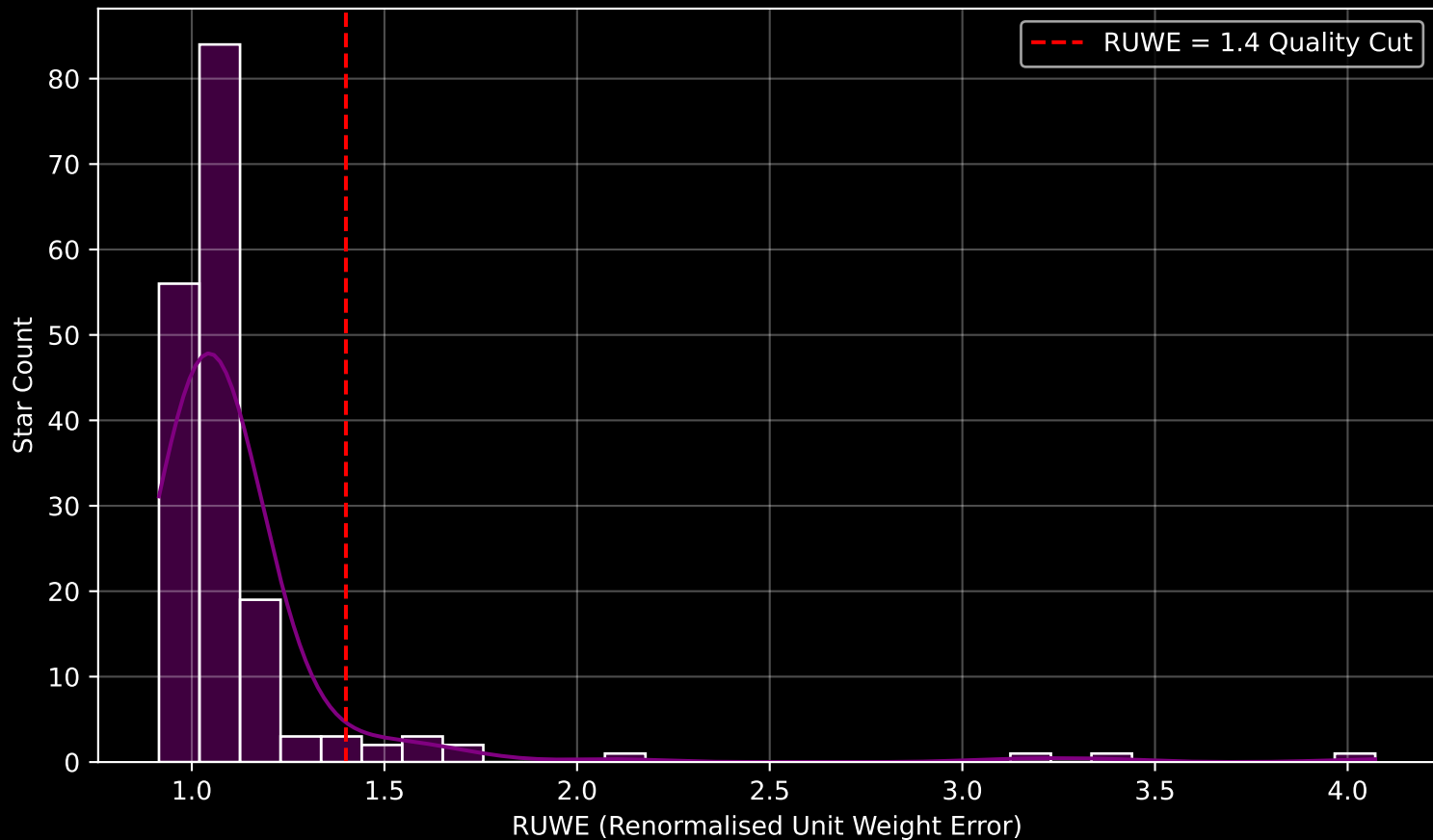
GAPOGEE DR17 Field [203-12] RUWE Distribution (n= 176)
