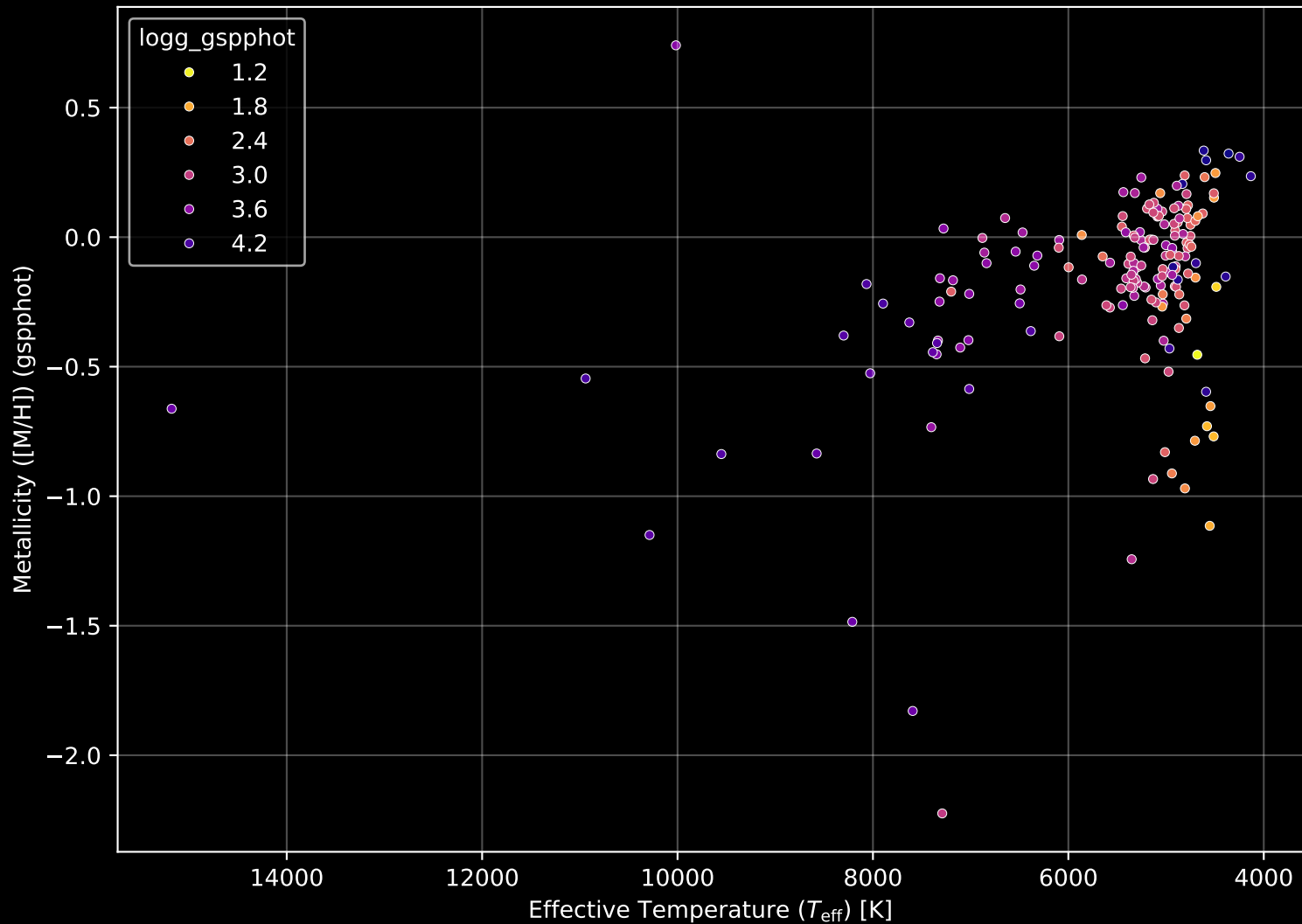
APOGEE DR17 Field: [203-12] Stellar Population Parameters (n= 177)
