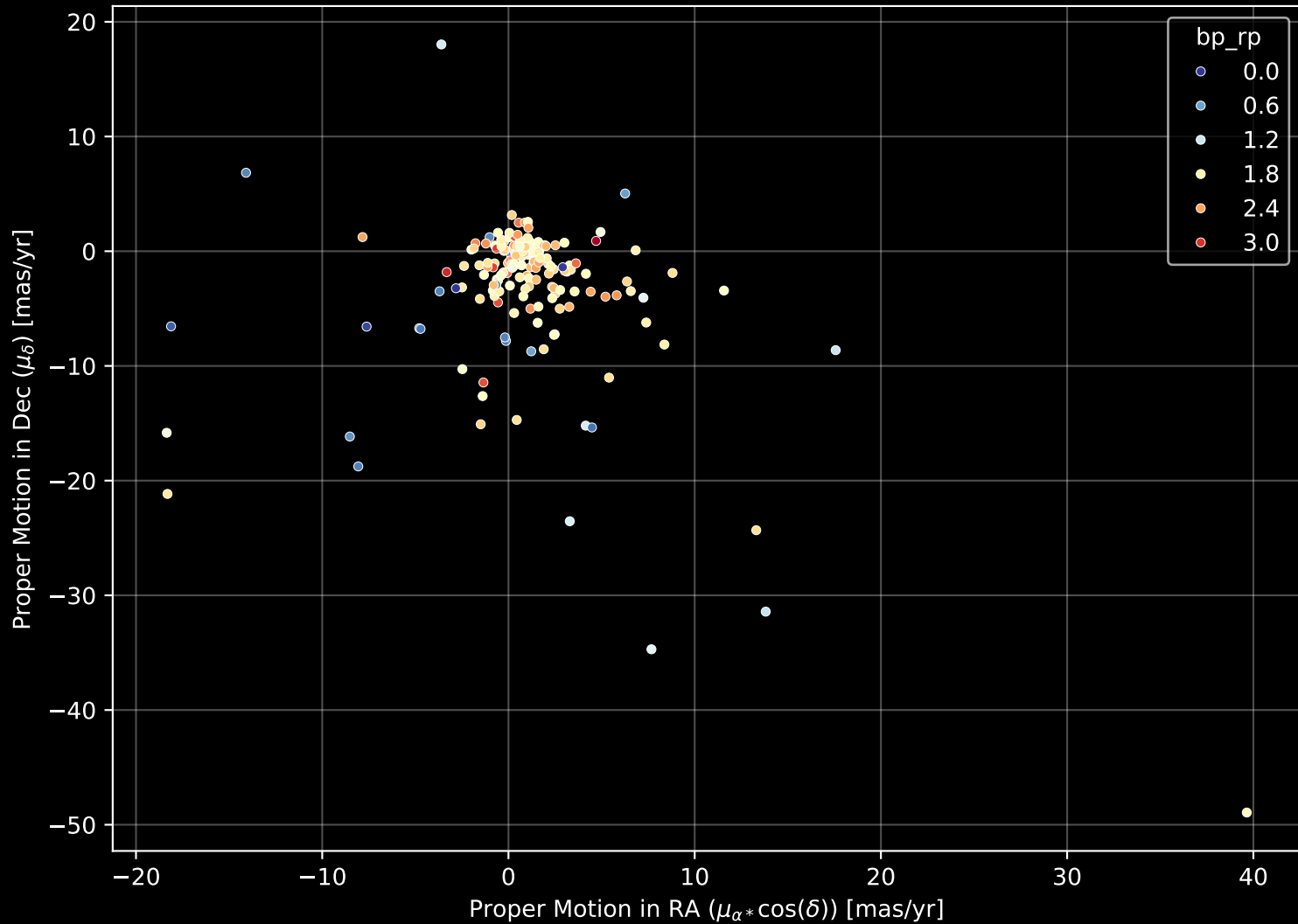
APOGEE DR17 Field: [203-12] Proper Motion Diagram (n= 177)
