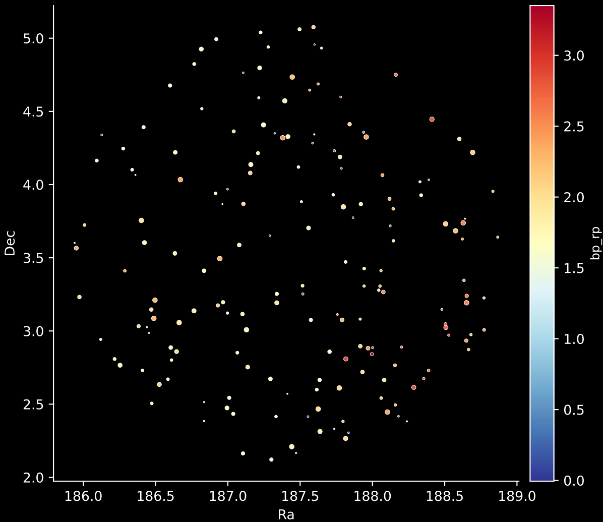
APOGEE DR17 Field: [203-12] Stars: 177
