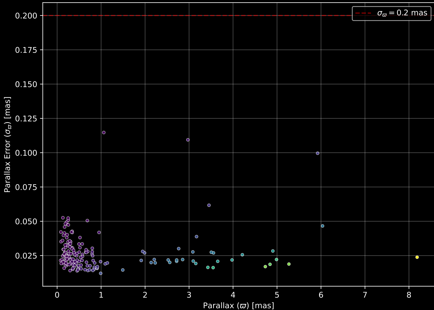
APOGEE DR17 Field: [203-12] Parallax Quality (n= 177)
