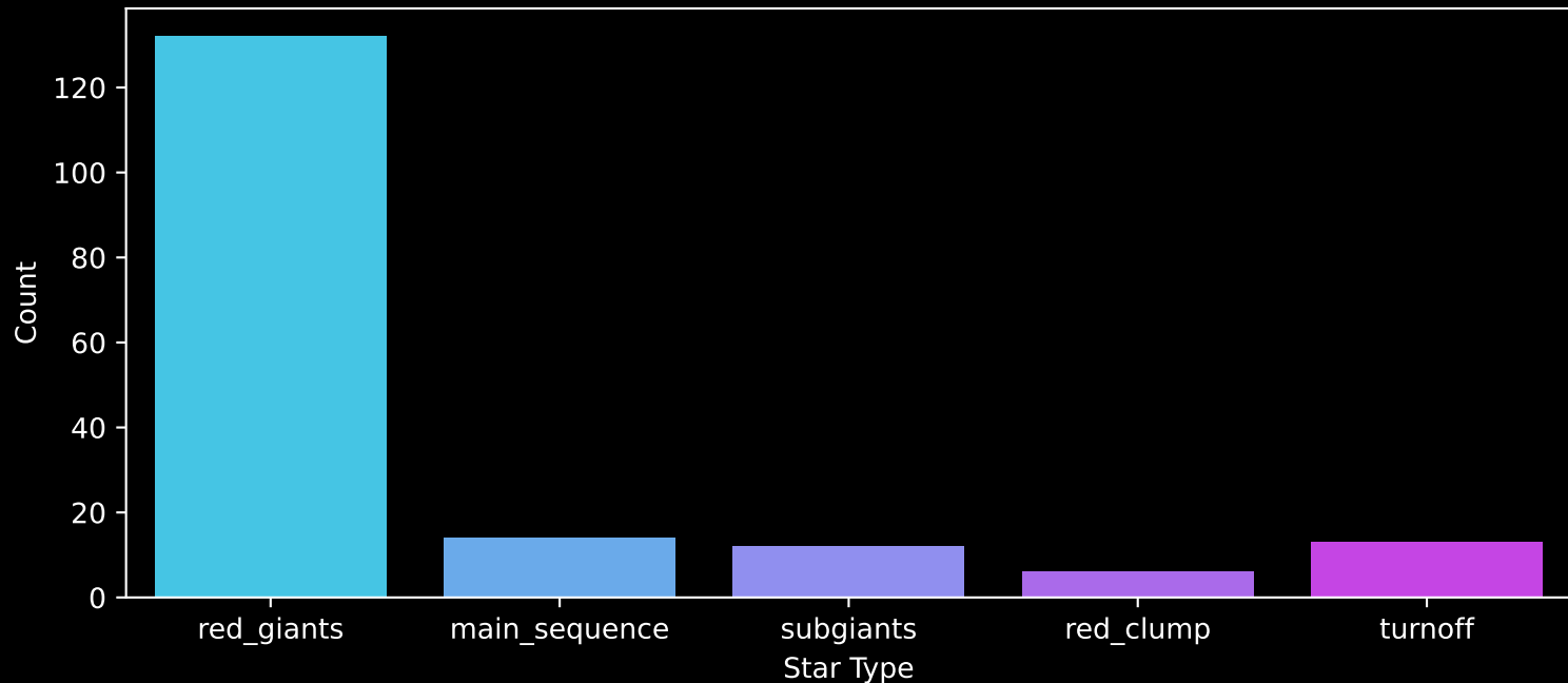
APOGEE DR17 Field: [203-12] Count plot of Star Type
